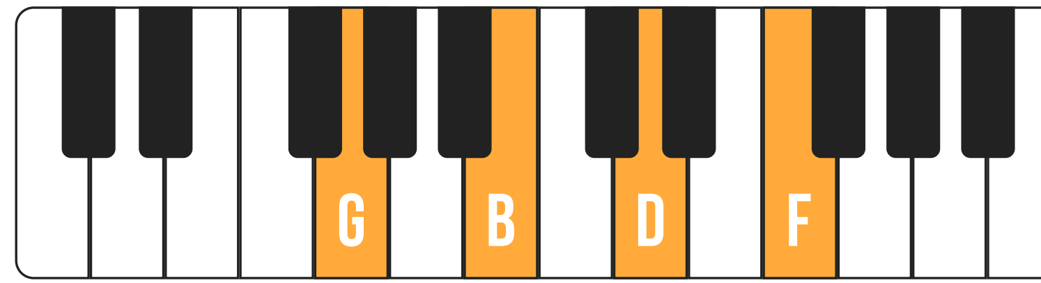
G dominant 7 (G7)
