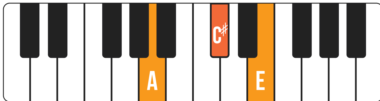
A Major (A)
